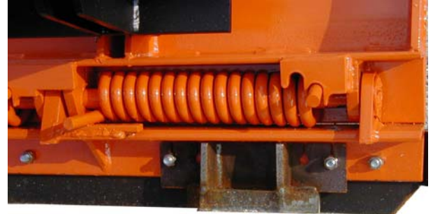
Trip edge mechanism as shown below.
